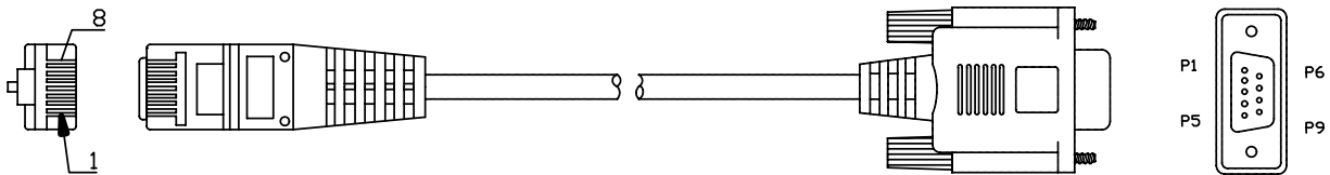
6P6C TO DB15P
