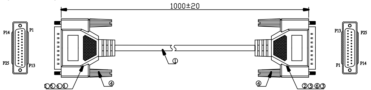
DB25/Plug TO DB25/Plug.
